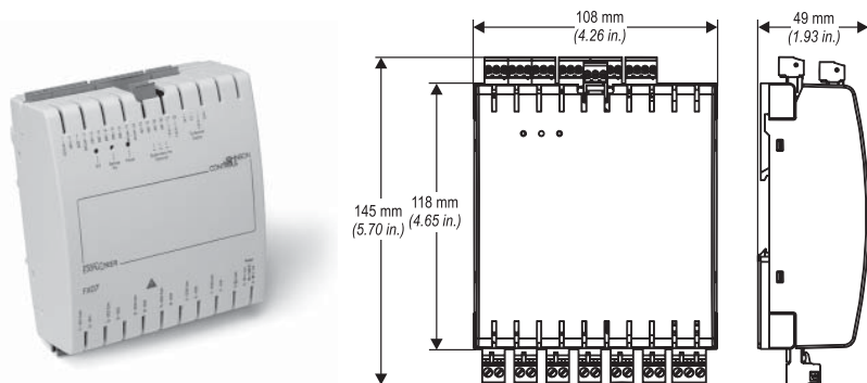
FX07 Field Controller Without Display Model Dimensions in mm (inches)
