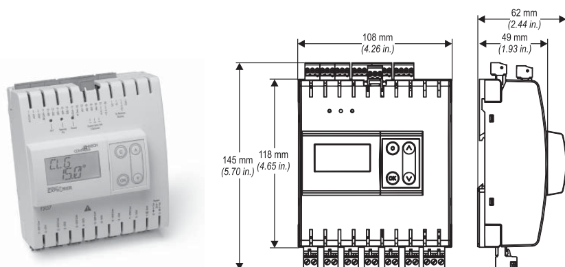
FX07 Field Controller Display Model Dimensions in mm (inches)
